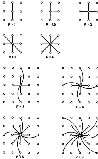
Fig. 2—Definition of redundancy level.
