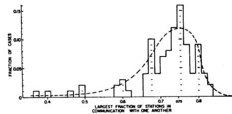
Fig. 7—Probability density distribution of largest fraction of stations in communication; perfect switching, R = 3 , 100 cases, 80 per cent node survival, 65 per cent link survival.
