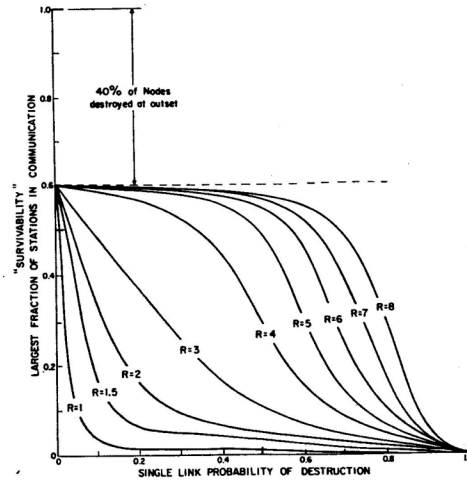
Fig. 6—Perfect switching in a distributed network: sensitivity to link destruction after 40 per cent nodes are destroyed.
